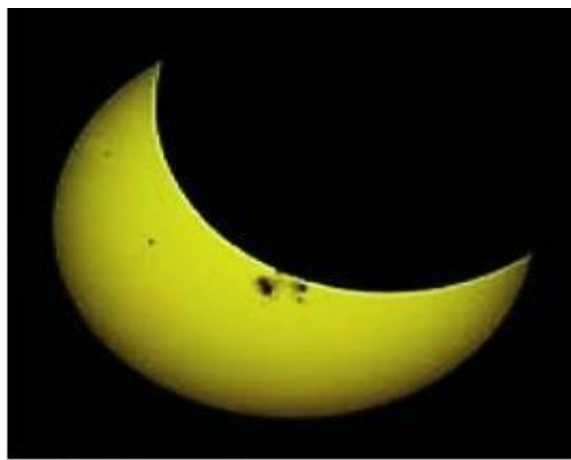
(b) Partial eclipse
